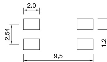
(PCB Pattern)
