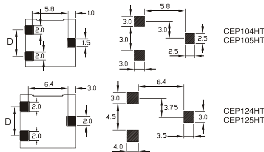
LAND PATTERN
