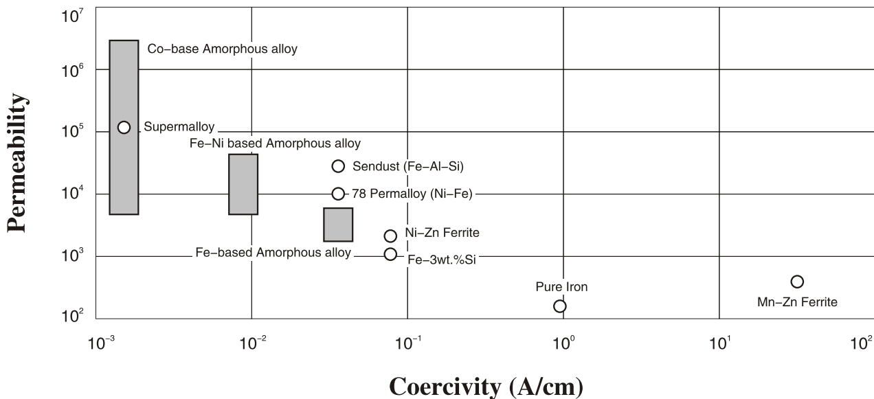
Permeability vs. Coercivity
