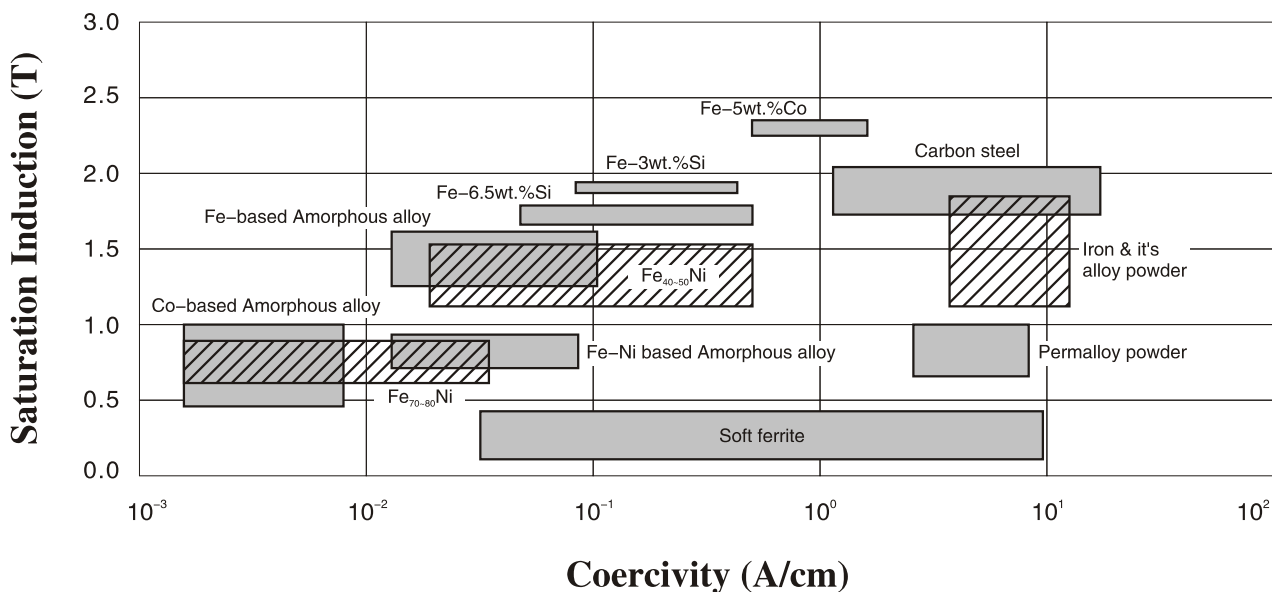
Saturation Induction vs. Coercivity
