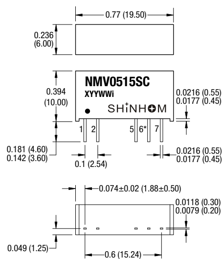
SIP package
